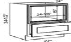
Built-in Microwave Base BMB27 - Includes Wood Trim Designed for fitting Countertop or Drawer Microwaves. The bottom trim may need to be cut out to fit full microwave drawer models.
