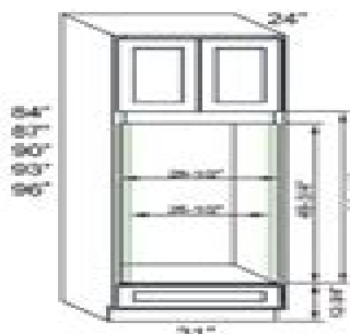
Oven & Microwave-Oven Combo Cabinets OC3184, OC3187, OC3190, OC3193, OC3196 Fit Both 27" and 30" wide ovens
