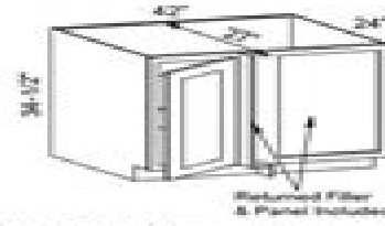
Base Blind Corner BBC42 - Interchangeable L & R Resize to BBC45 by + WDR19.5x30 Resize to BBC46 by + WDR21.5x30
