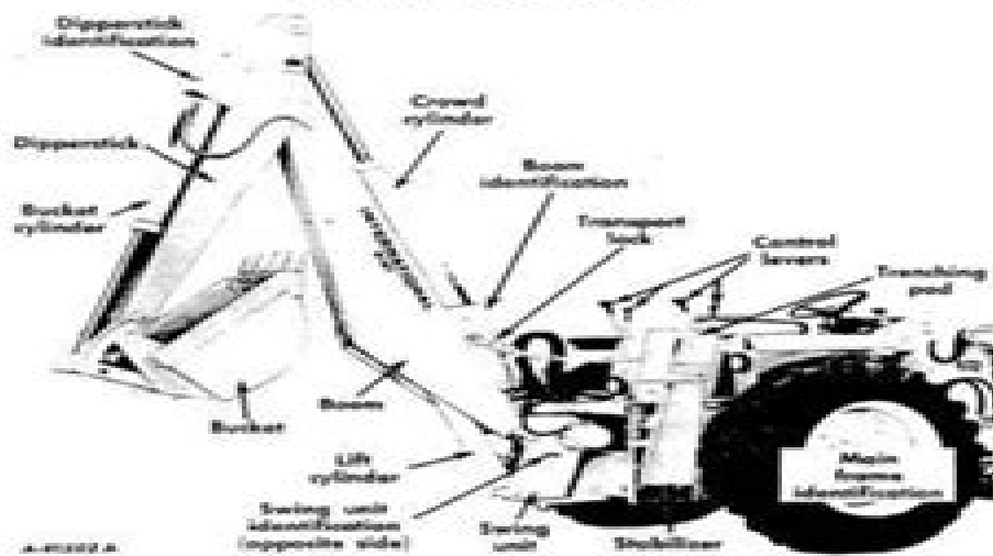
Location of units and parts. International 3021 Backhoe shown as International 3456 Loader Tractor.
