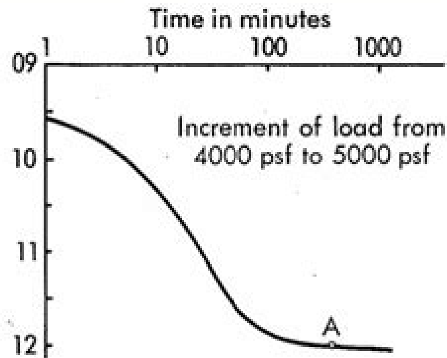
a. Time-settlement curve for one load increment
