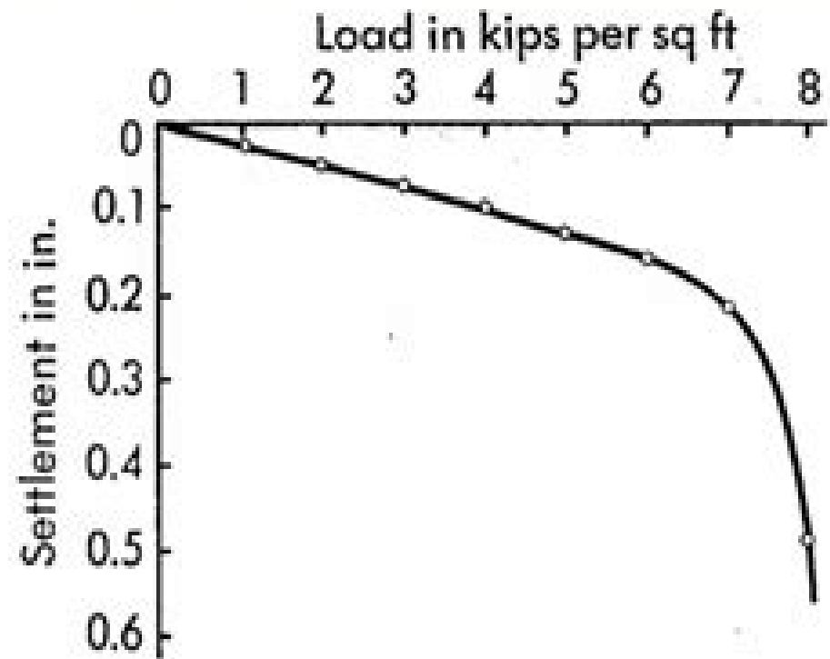
b. Load settlement curve
