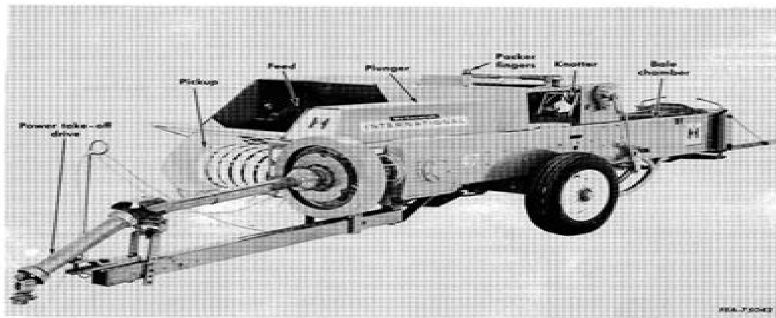
Illustr. 1. Left side view of the No. 47 Baler with power take-off.
