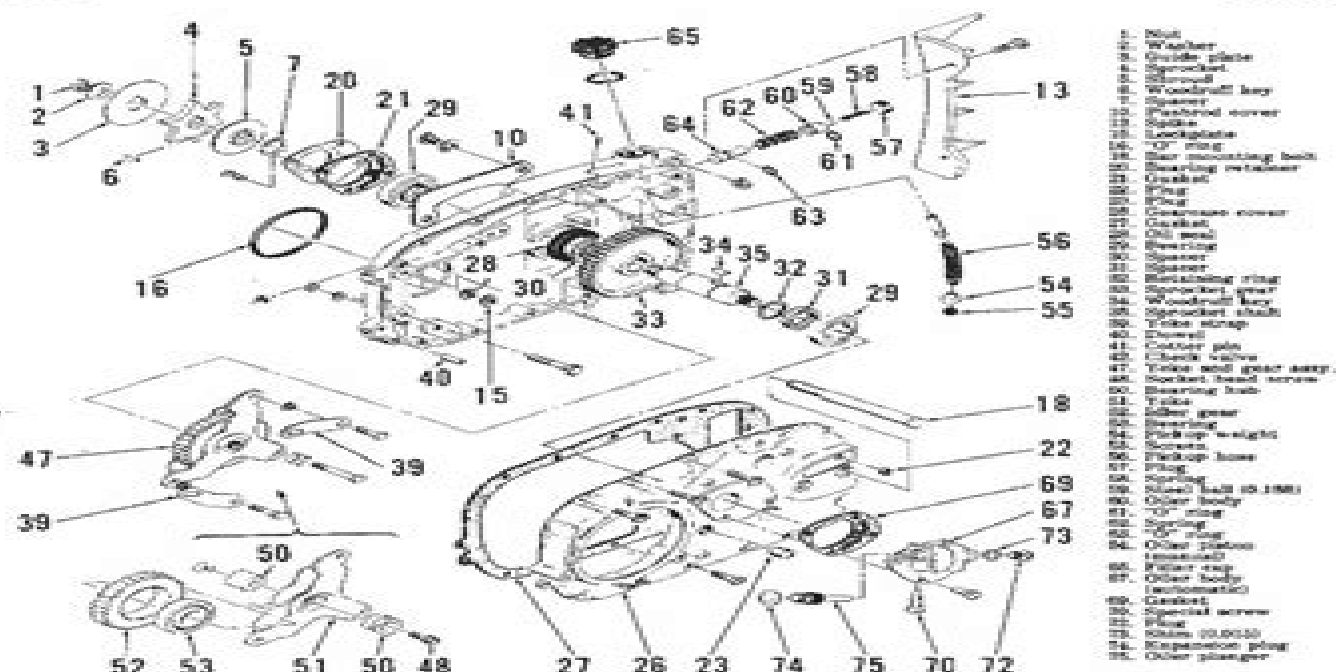
Fig. MCS-24—Exploded view of transmission used on Models 895 and 895C. Input gear is part of clutch drum (36—Fig. MCS-21). Shim (73) is 0.015 thick.
