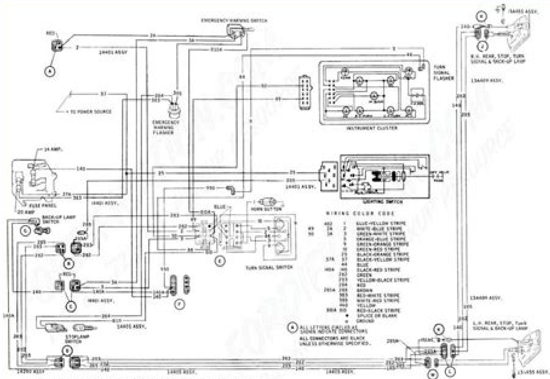
LAMP WIRING DIAGRAM F-250, F-350 Platform and Stake Models
