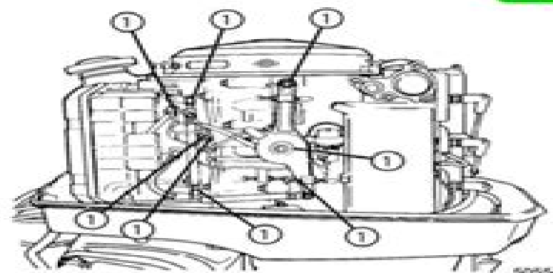
1 - Throttle/Shift Linkage Pivot Point Lubrication
