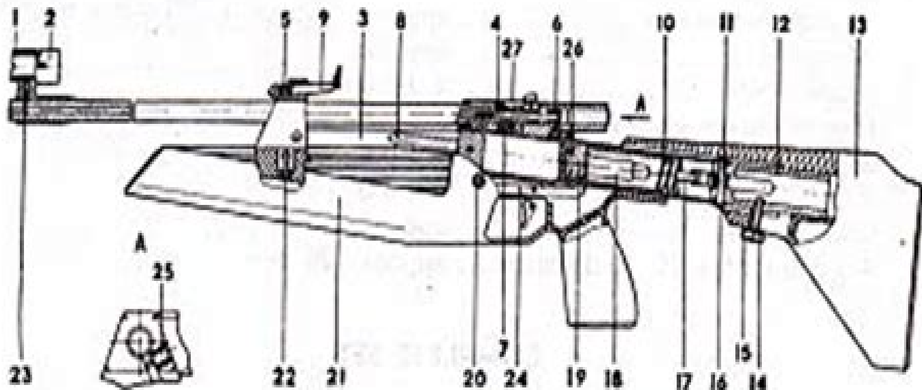
Fig.1. Scheme of the IZH-61 mechanisms
