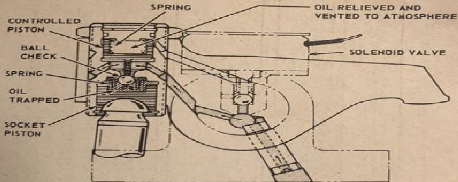
Oil Flow Through Lash Adjuster-Brake On (© Mack Trucks Inc.)
