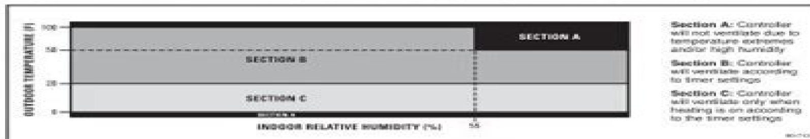
FIGURE 1 – OPERATING LIMITS
