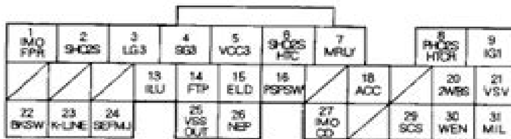
Wire side of female terminals
