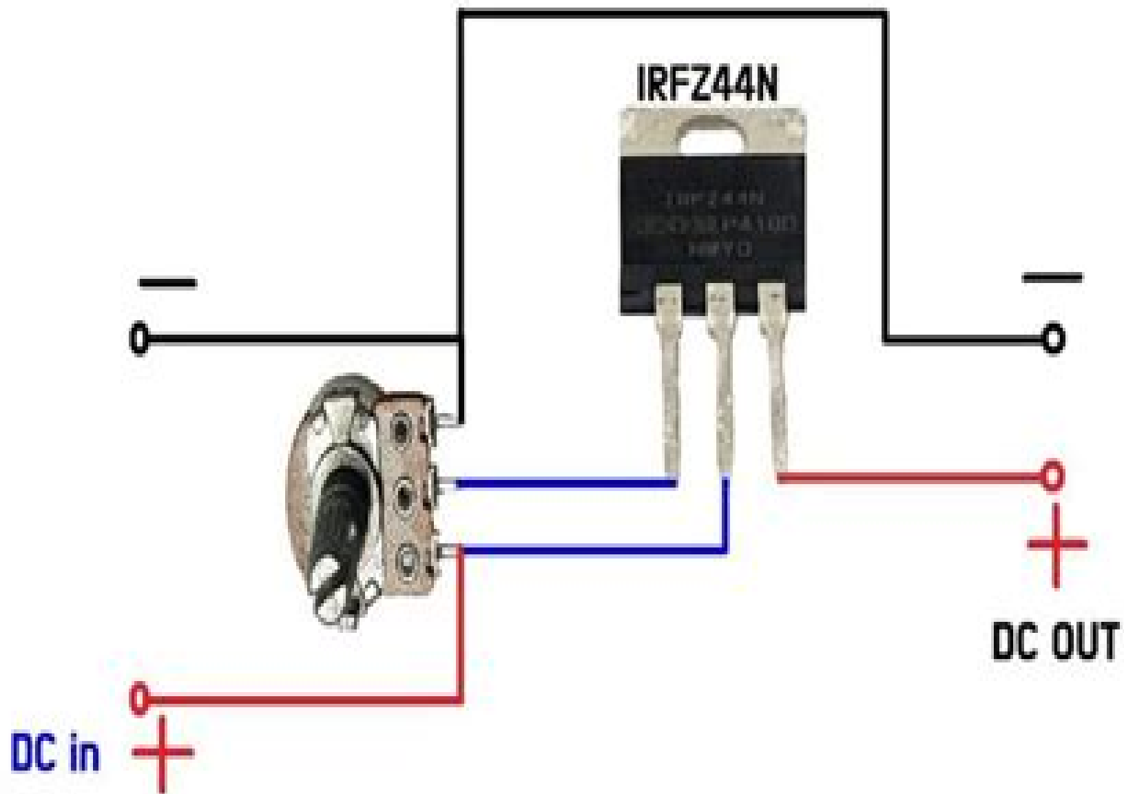
DIY IRFZ44N MOSFET Voltage Regulator
