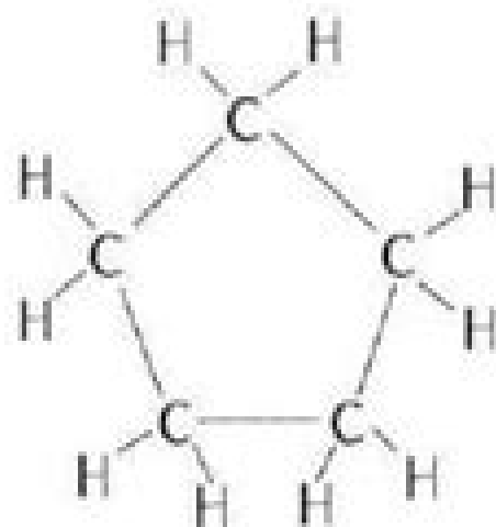
Cyclopentane
