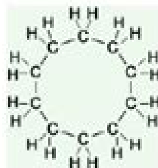
Cyclodecane
