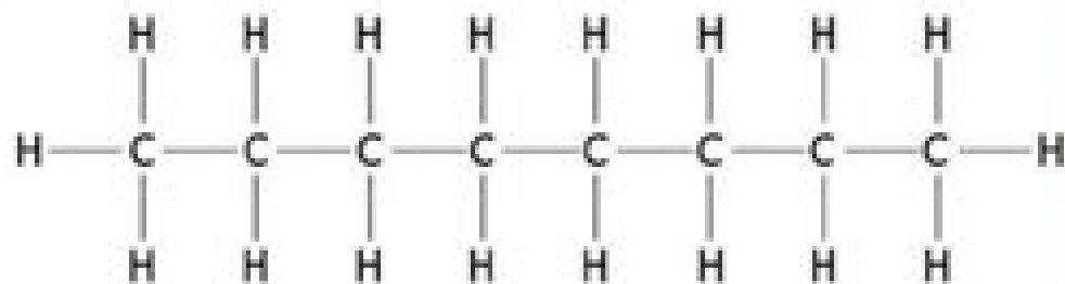
Octane
