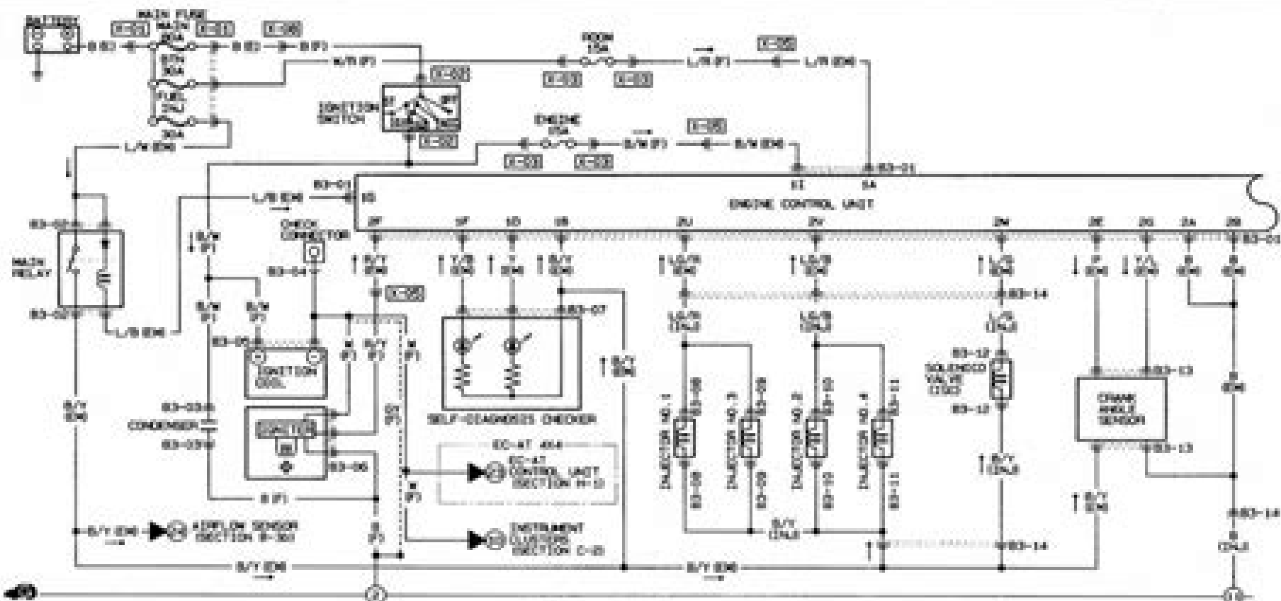
B3-01 ENGINE CONTROL UNIT (EH)
