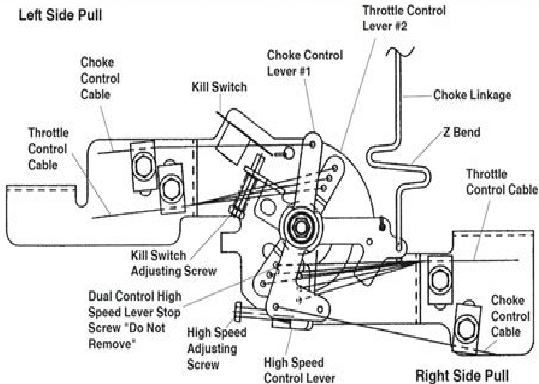
Figure 5-87. Governor Control Connections.
