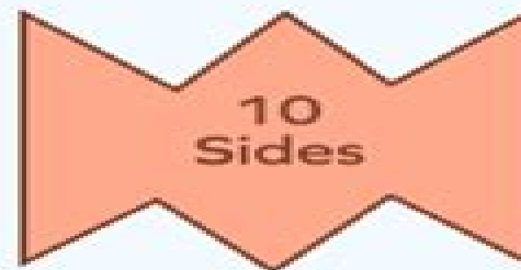
Irregular Decagon
