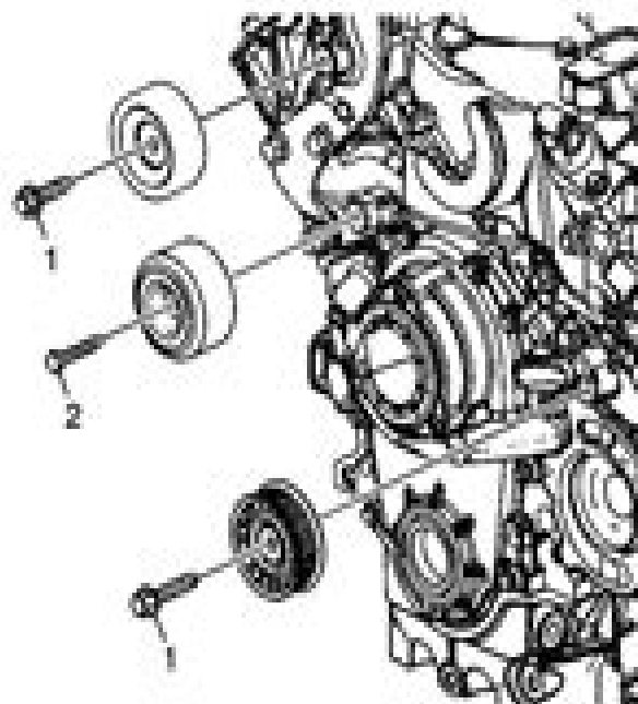
Fig. 627: Identifying Idler Pulley Bolts & Pulleys Courtesy of GENERAL MOTORS CORP.
