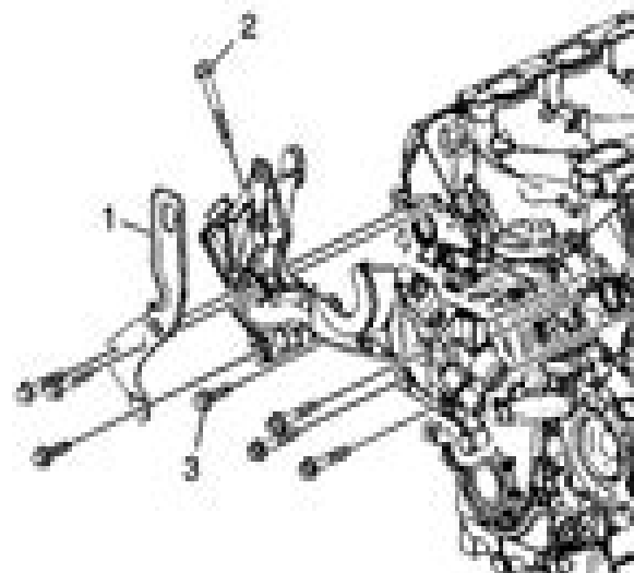
Fig. 628: Identifying Coolant Crossover Pipe Bolts Courtesy of GENERAL MOTORS CORP.
