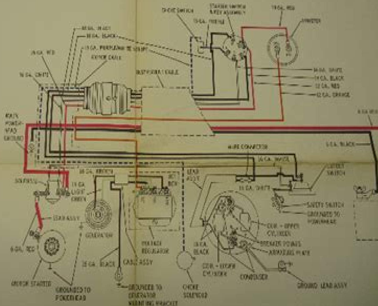
P71 WIRING DIAGRAM 40 HP MODEL (WITH GENERATOR)
