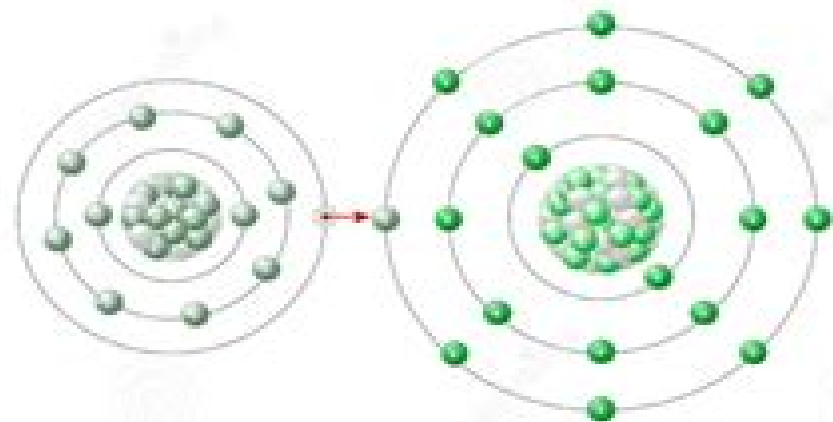
Ionic bond
