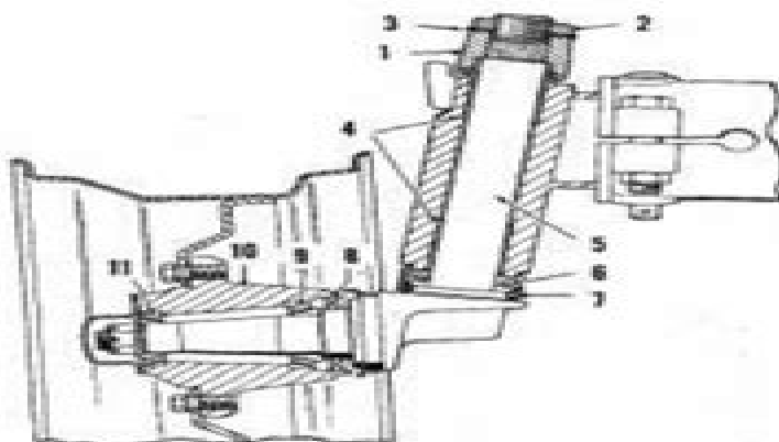
Fig. 5 - Cross sectional view of typical steering knuckle used on all models.
