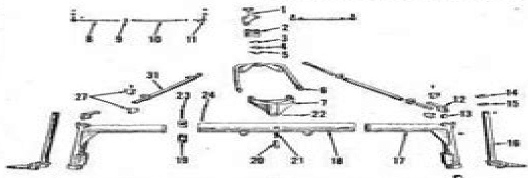
Fig. 4 - Exploded view of adjustable wide front axle used on Models 986 and 1086 Hi-Clear tractors.
