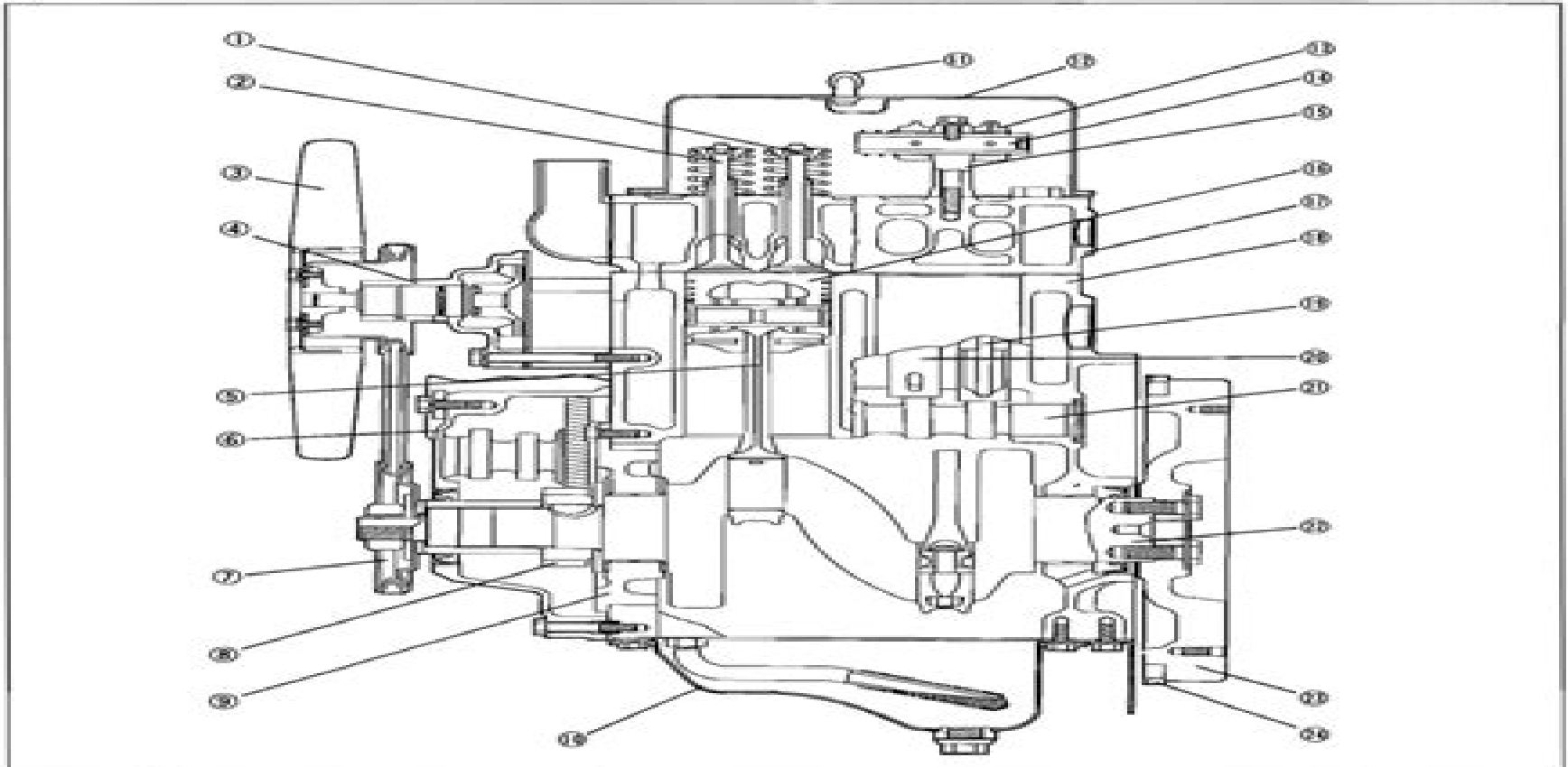
(5) Cross section of KE70
